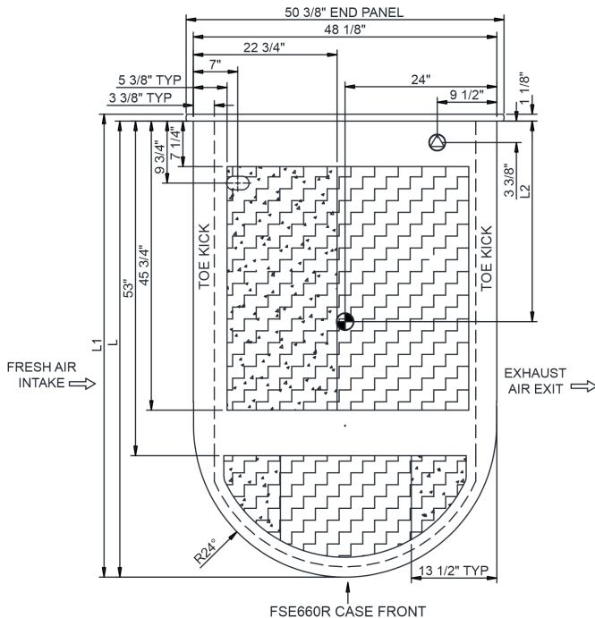
PLAN VIEW
