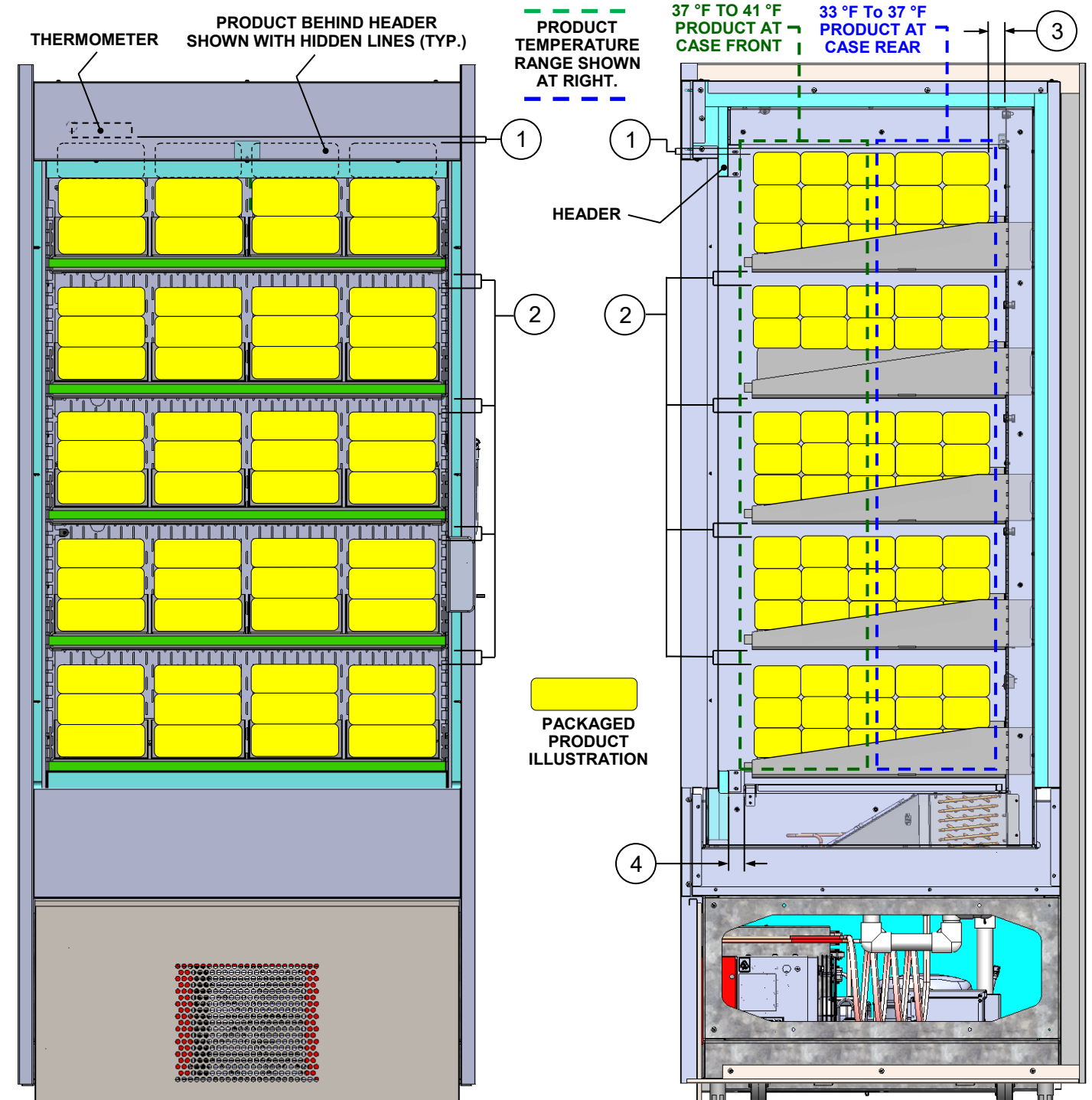
MODEL BD3632IS SHOWN ABOVE. CASE IS PARTIALLY DISASSEMBLED, CROSS-SECTIONED AND PACKAGED PRODUCT LADEN FOR ILLUSTRATIVE PURPOSES
